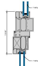
HORIZONTAL INTEGRAL MULLION (PANEL/FIXED) ③ S = 1'0"
