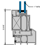
② STANDARD SILL 6\" = 1'-0"
