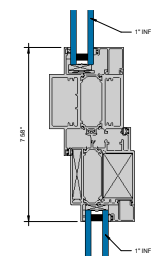
HORIZONTAL INTEGRAL MULLION ③ (PANEL/FIXED) 6" = 1'-0"
