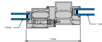
VERTICAL INTEGRAL MULLION (PANEL/FIXED) ② S = 1'0"
